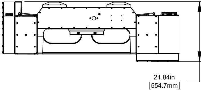
Front View Platter Rotated 90° to Base
